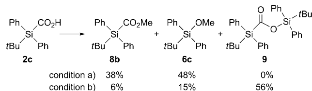
Scheme 4. Methyl esterification of silacarboxylic acid 2c : a) cat. H 2 SO 4 , MeOH, reflux; b) MeOH, DCC, cat. DMAP, CH 2 Cl 2 , RT. DCC = N,N' -dicyclohexylcarbodiimide, DMAP = 4-(dimethylamino)pyridine.
