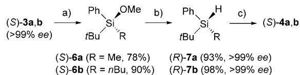
Scheme 2. Preparation of nonracemic chiral chlorosilanes 4 : a) MeI, KH, DMF, RT; b) LiAlH 4 , Et 2 O, reflux; c) (PhCO 2 ) 2 (10 mol %), CCl 4 , reflux. DMF = N,N -dimethylformamide.
