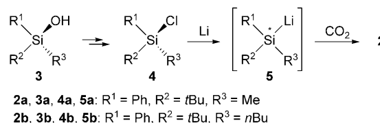
Scheme 1. Strategy for the asymmetric synthesis of chiral silacarboxylic acid.
